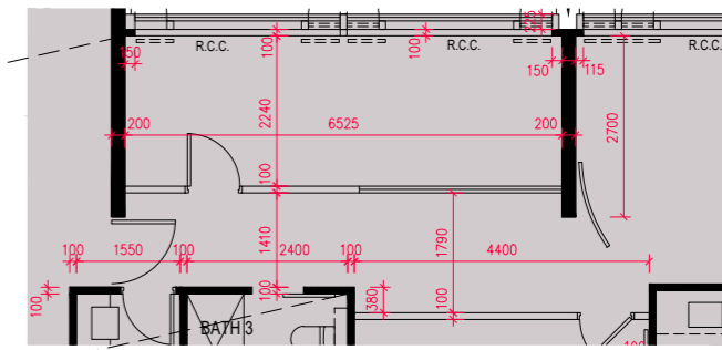
20/F PART PLAN IN "AS-IS" LAYOUT 20樓現狀部分平面圖
