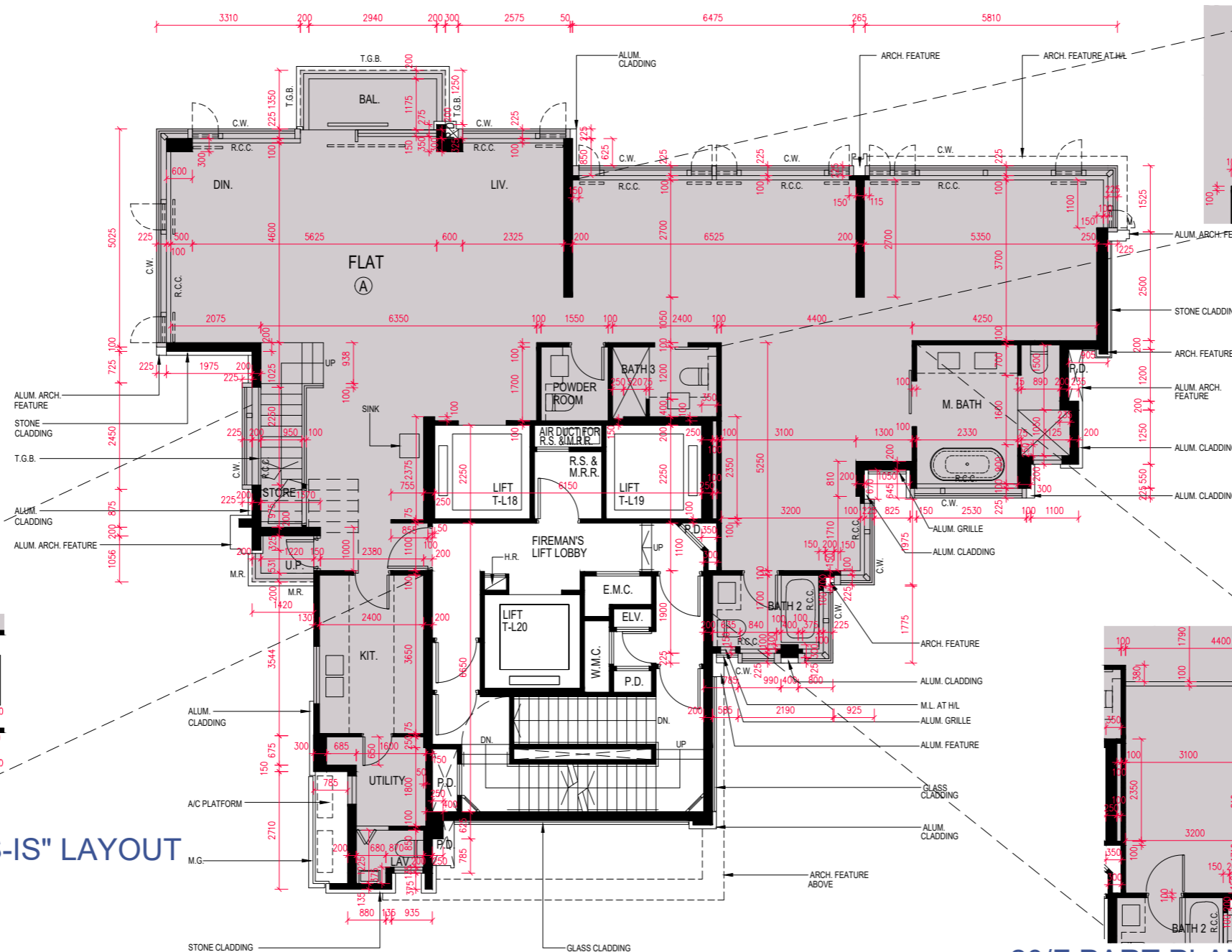
20/F PART PLAN IN "AS-IS" LAYOUT 20樓現狀部分平面圖
