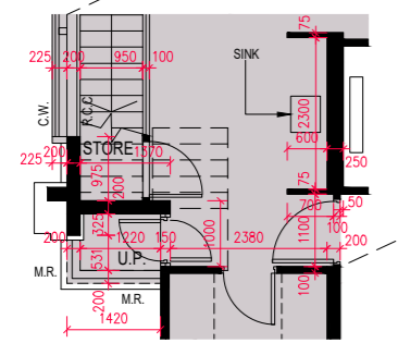
20/F PART PLAN IN "AS-IS" LAYOUT 20樓現狀部分平面圖
