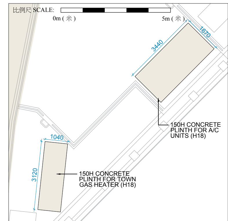
18 號洋房地下主層部分平面圖 Part Plan For House 18 Master Ground Floor Plan
