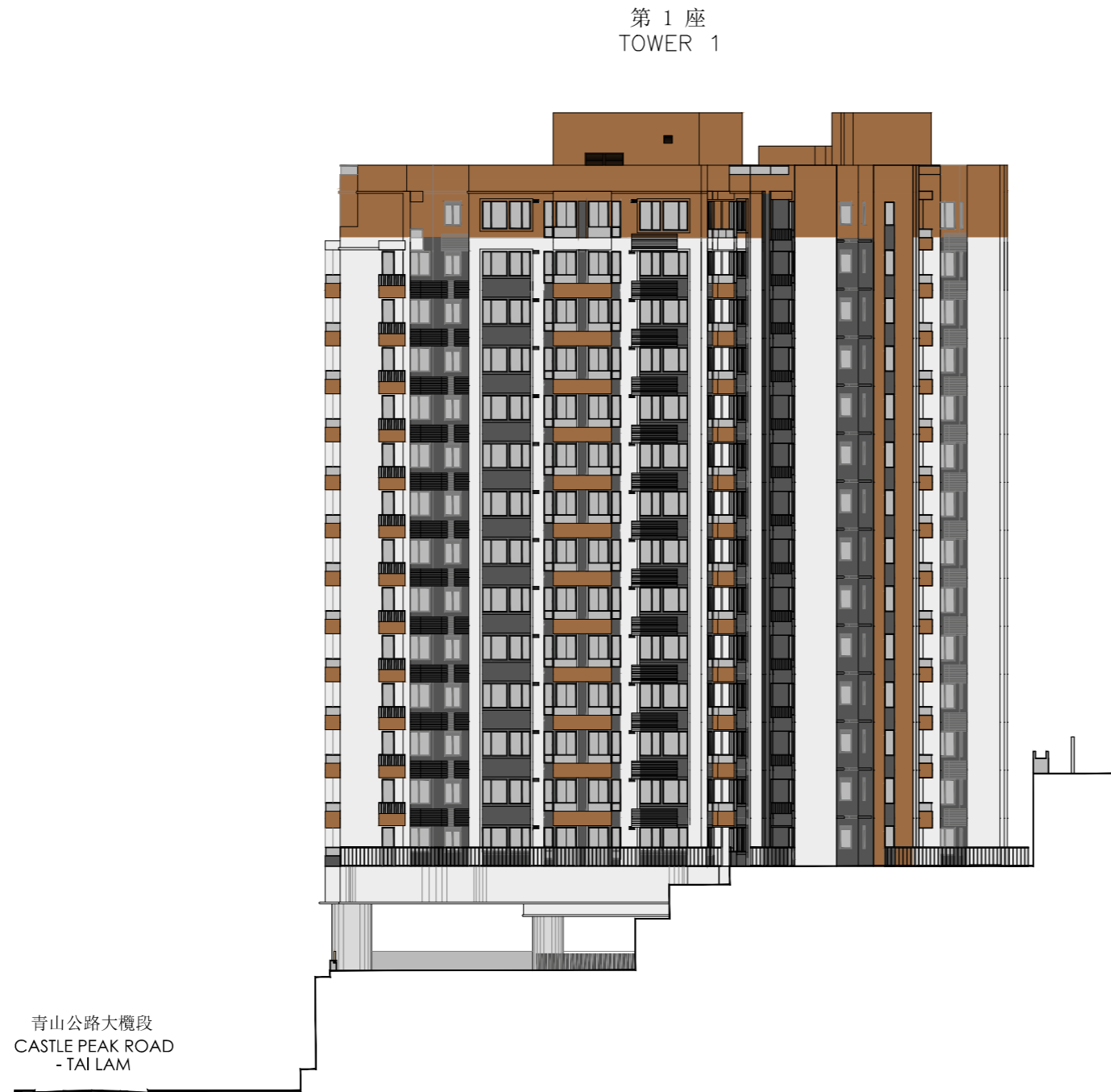
立面圖4 Elevation plan 4
