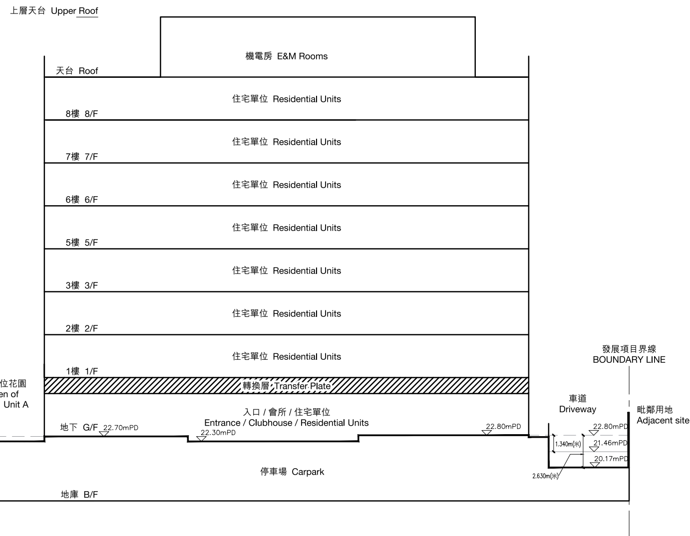
橫截面圖B-B Cross-Section Plan B-B
